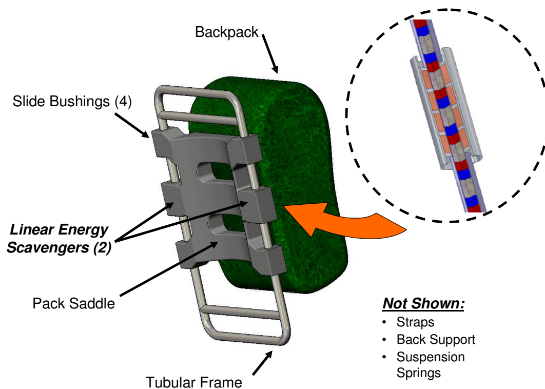
Figure 14. Backpack with Integrated Miniature Linear Electric Generators
