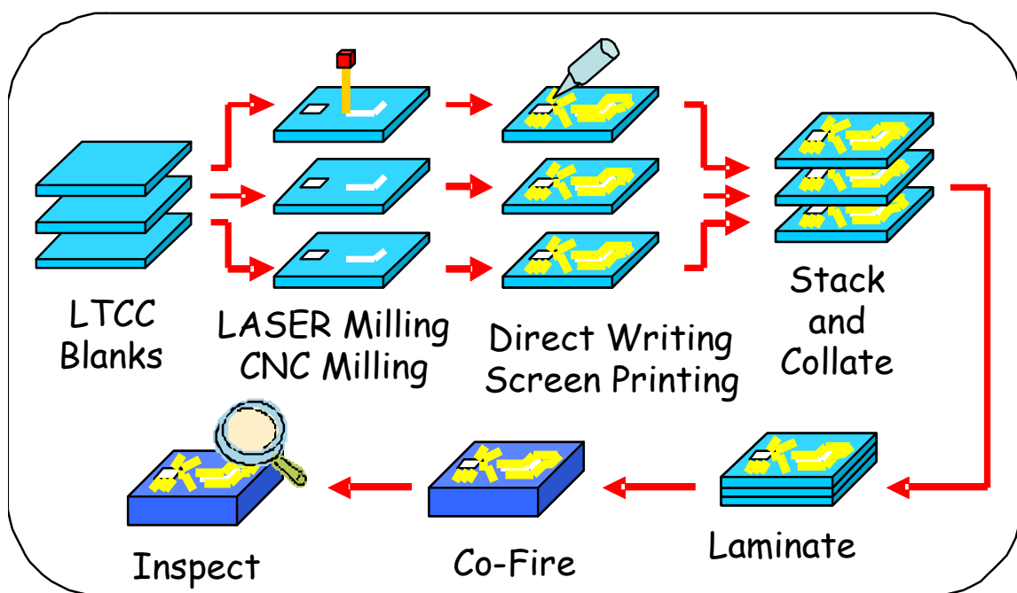
Figure 9. LTCC Process Flow [11]
