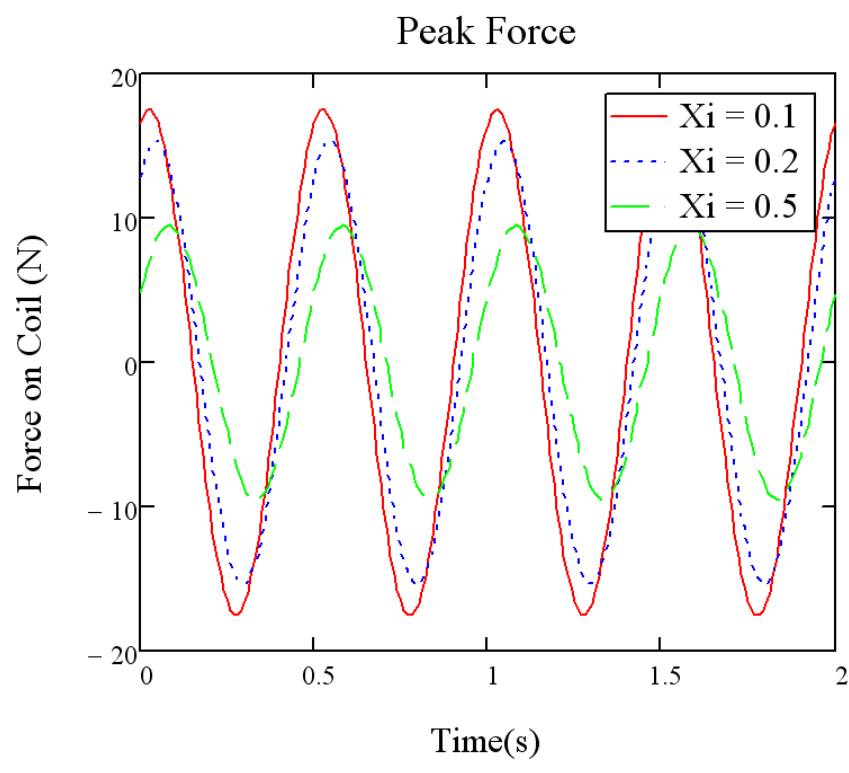
Figure 24. Peak Force from Coil
